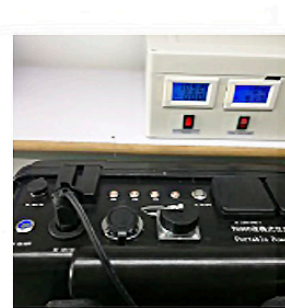
8.3 DC 48V output testing
